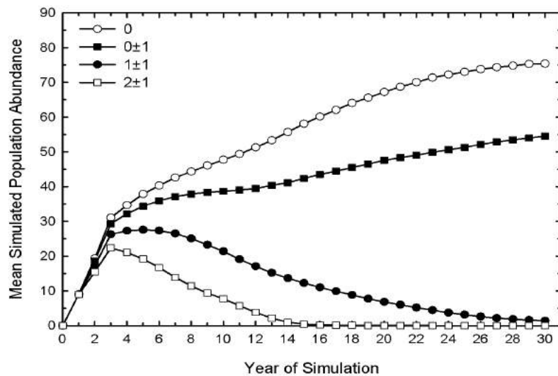
Figure 41. Mean abundance trajectories for a simulated Burachapori Wildlife Sanctuary population of greater one-horned rhino with translocation of animals from Kaziranga NP in years 1, 2 and 3. Top panel: 6 animals (3 female, 3 male) added each year. Middle panel: 9 animals (6 female, 3 male) added each year. Bottom panel: 15 animals (9 female, 6 male) added each year. Within each panel, the graph legend indicates the number of animals of each gender that are removed by poaching each year of the simulation. See accompanying text for more information on model structure and interpretation.
